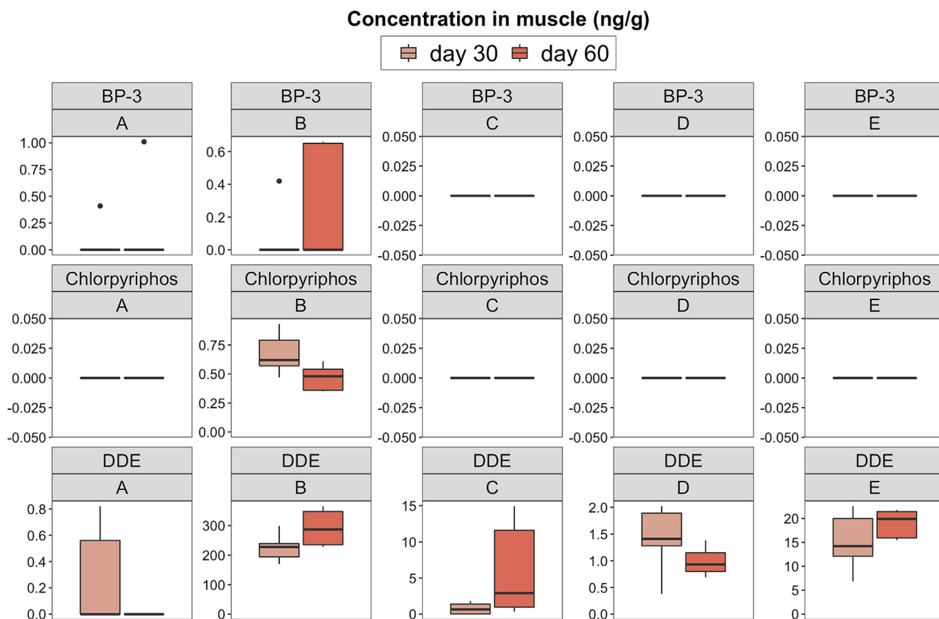
Fig. 5. Concentration of chemical pollutants (ng/g) in Dicentrarchus labrax muscle after 30 and 60 days feeding each treatment.
