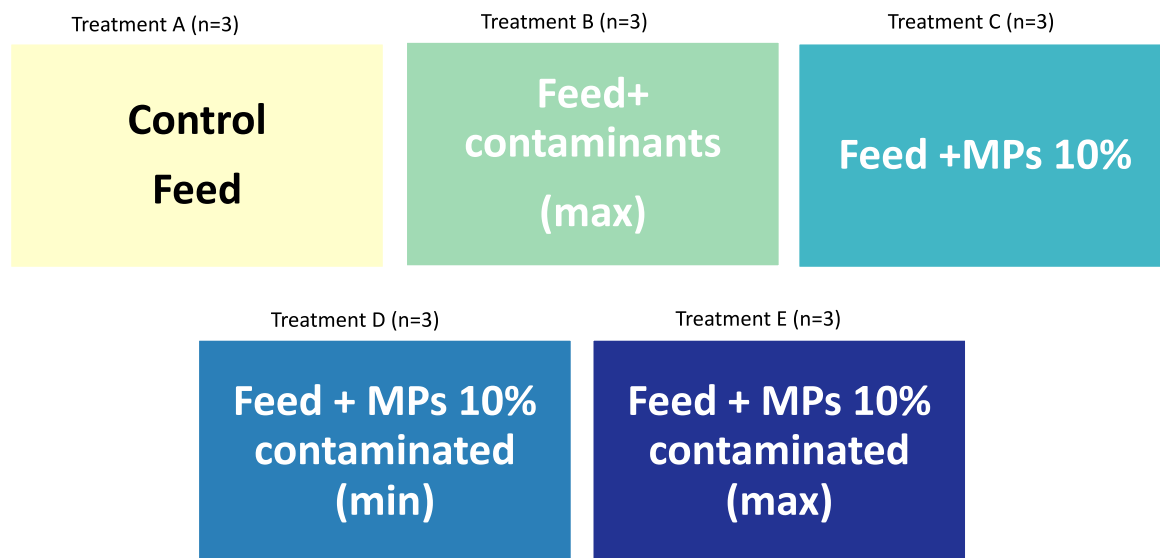
Fig. 1. Composition of each diet A) Feed; B) Feed plus BP-3, CPS and DDE-p,p' at maximum; C) Feed plus 10 % virgin MPs; D) Feed plus 10 % MPs contaminated at minimum; E) Feed plus 10 % MPs contaminated at maximum.
