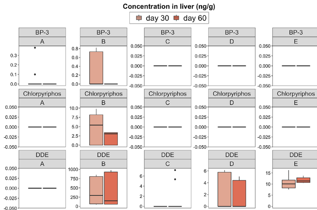
Fig. 4. Concentration of chemical pollutants (ng/g) in Dicentrarchus labrax liver after 30 and 60 days feeding each treatment.
