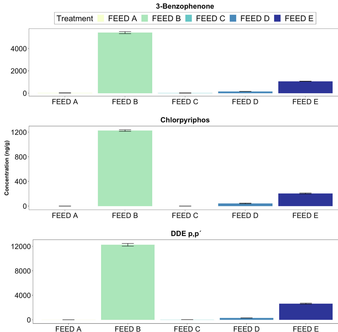
Fig. 3. Concentration of chemical pollutants (ng/g) (mean \pm SD) in each treatment: Feed A (Control); Feed B (feed plus BP-3, CPS and DDE-p,p' at maximum concentration); Feed C (feed plus 10 % virgin MPs); Feed D (feed plus 10 % MPs contaminated with BP-3, CPS and DDE-p,p' at minimum concentration); Feed E (feed plus 10 % MPs contaminated with BP-3, CPS and DDE-p,p' at maximum concentration).
