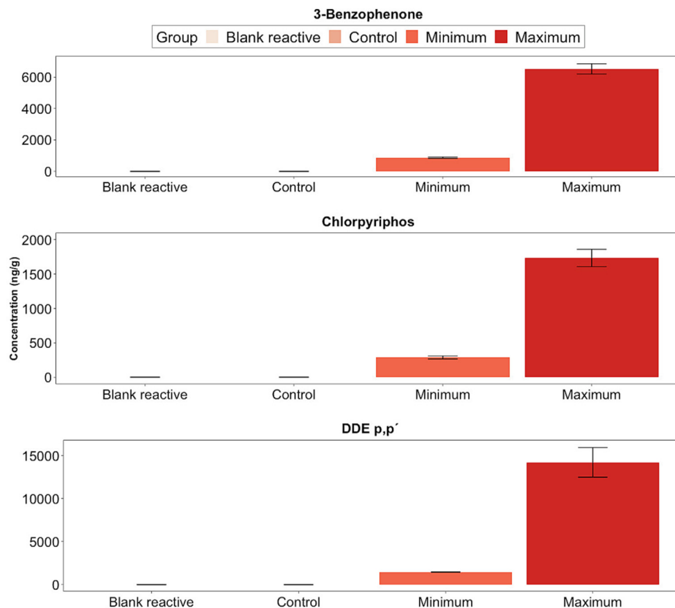
Fig. 2. Concentration in ng/g of BP-3, CPS and DDE-p,p' in MPs in blank reactive, control, minimum contamination, and maximum contamination.
