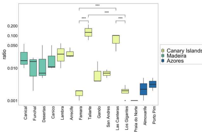
Fig. 3c. Ratio Microplastics/Zooplankton abundance. Significant differences between locations within each archipelago are shown *** ( p < 0.001 ), ** ( p < 0.05 ), * ( p < 0.01 ).
